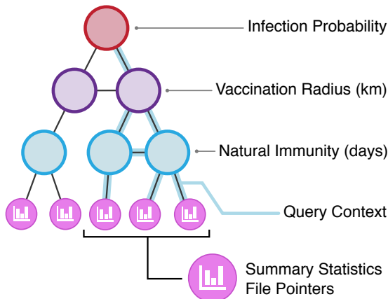
Fig. 4. An example analytic base tree with three feature layers. A query context, shown with highlighted edges, prunes the feature space to select particular sets of files or summary statistics.
