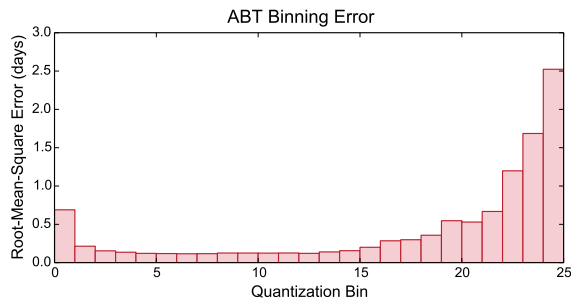
Fig. 6. Root-mean-square error for each range of values created by our autonomous binning algorithm. Frequently-observed values are placed in the smallest ranges, resulting in higher accuracy.
