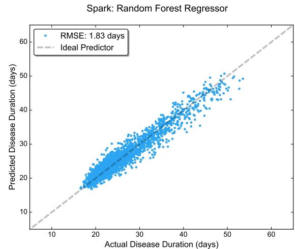
Fig. 9. Prediction performance of a random forest model generated in Spark with our RDD export functionality.
