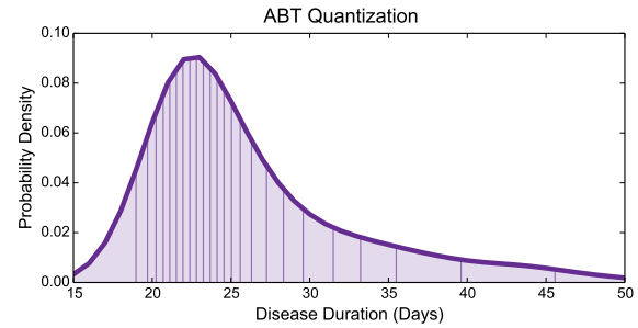
Fig. 5. A demonstration of the autonomous binning supported by analytic base trees. Feature values with higher probabilities are placed in smaller (and therefore more accurate) bins.
