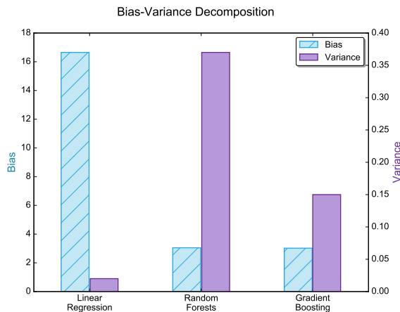
Fig. 8. Bias-variance decomposition for three of the built-in models supported by TRIDENT.
