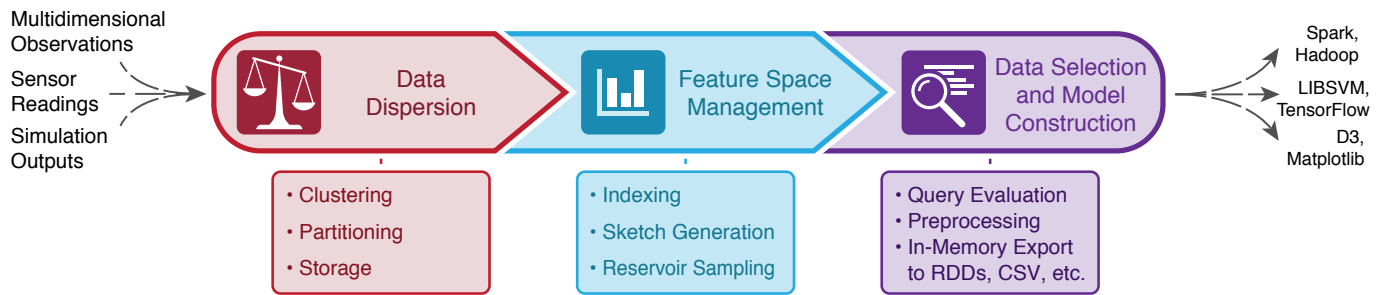
Fig. 1. TRIDENT architecture: multidimensional records are partitioned and indexed for subsequent analysis through expressive queries. Once records of interest are located and transformed, they are exported in memory to a variety of computation engines' native data structures.
