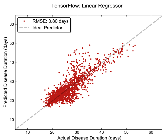
Fig. 10. Prediction performance of a linear regression model generated in TensorFlow with our TFRecord export functionality.
