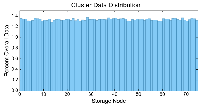
Fig. 2. Distribution of data with our cluster-based locality-sensitive hashing scheme across 75 storage nodes.
