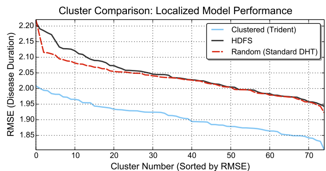
Fig. 3. Gradient-boosted decision tree models built in parallel with TRIDENT compared to models generated over randomly-placed data on a traditional DHT. Controlling the placement of data results in a 5–9% improvement in prediction accuracy.
